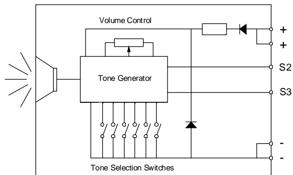
Fig 1 Simplified block diagram
